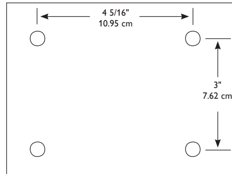
Mounting Pattern
